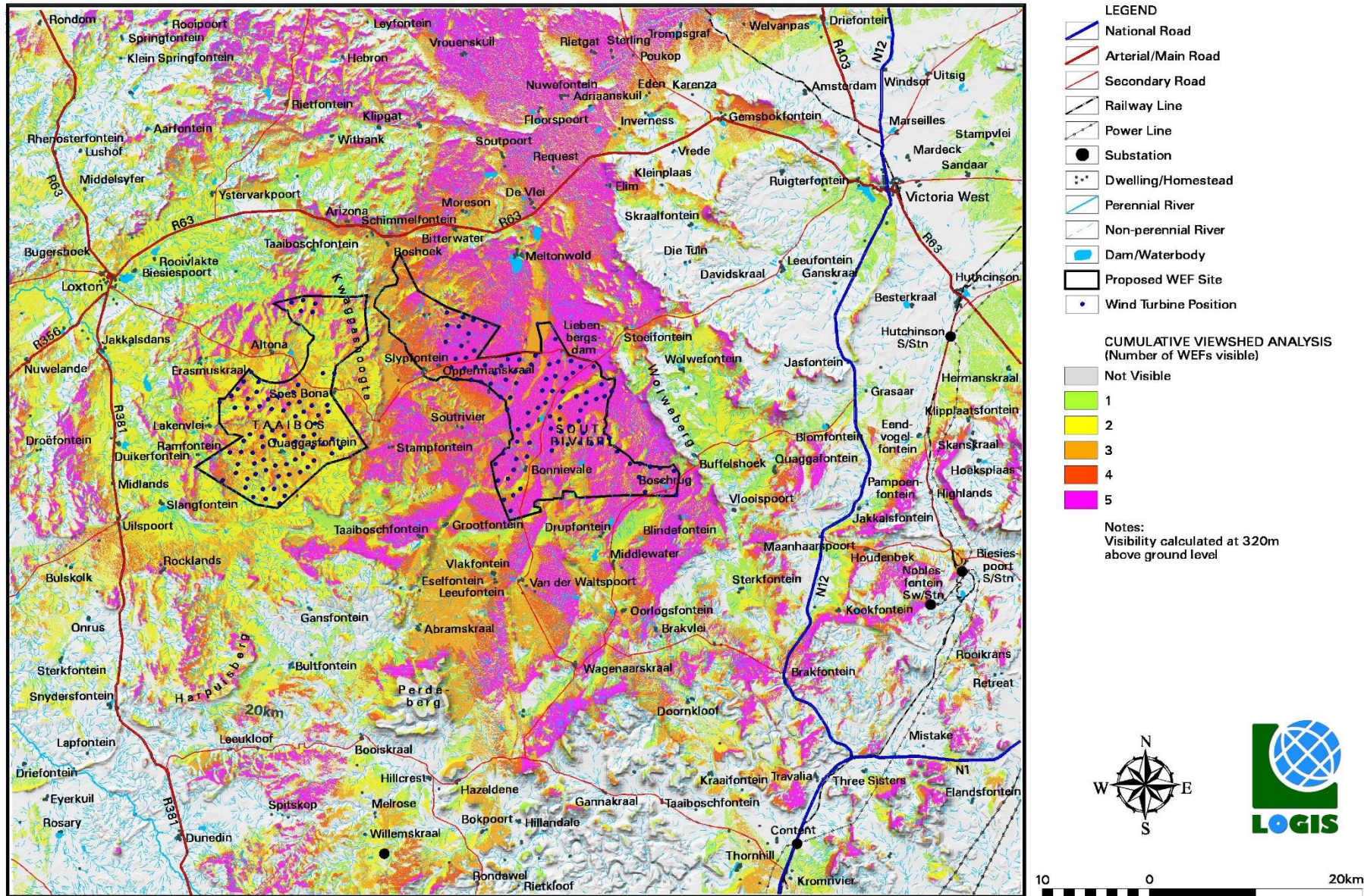
Map 5: Cumulative viewshed analysis for Victoria West WEF cluster
