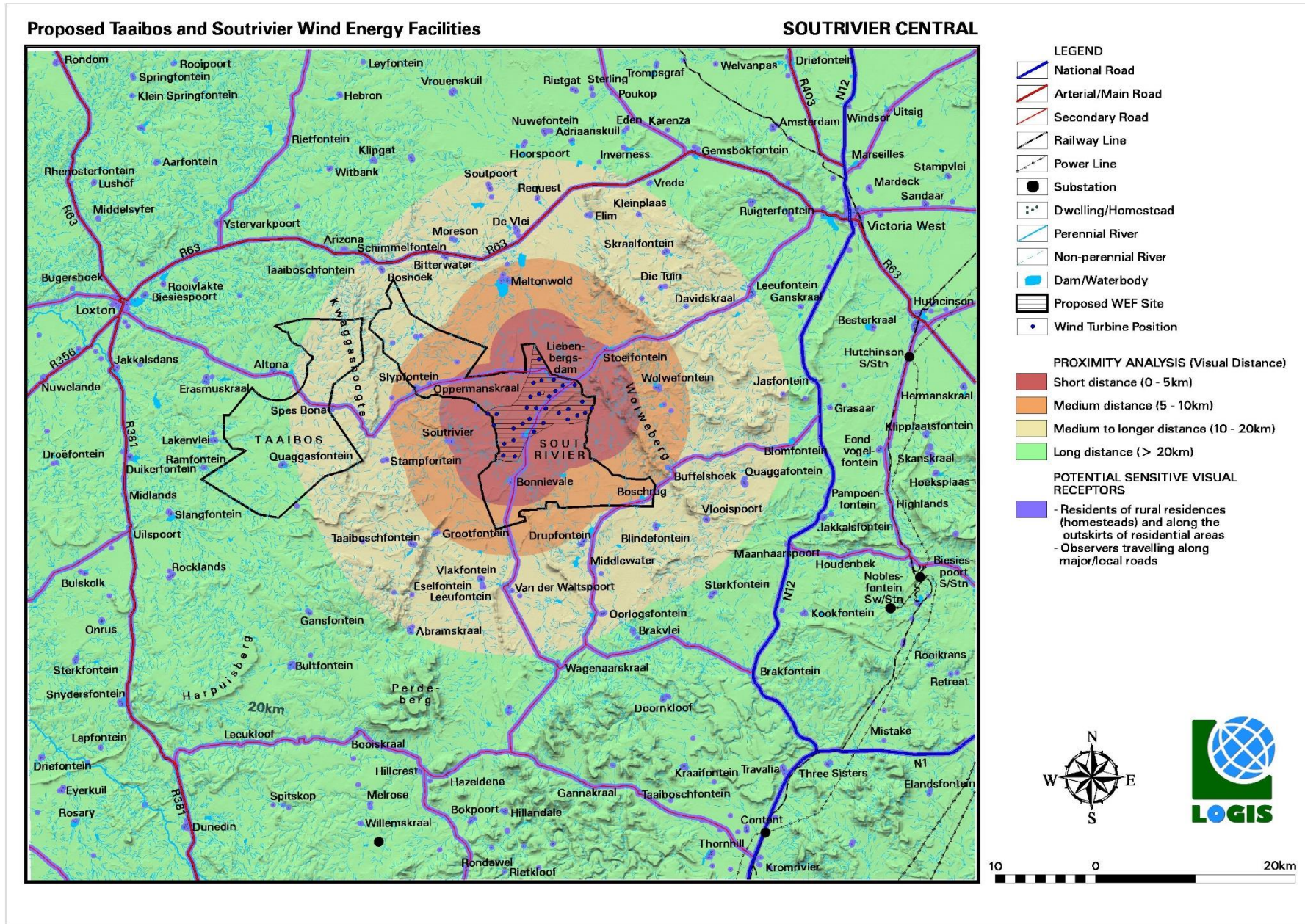
Map 3: Visual proximity analysis, observer sensitivity and proximity of the proposed Soutrivier Central WEF
