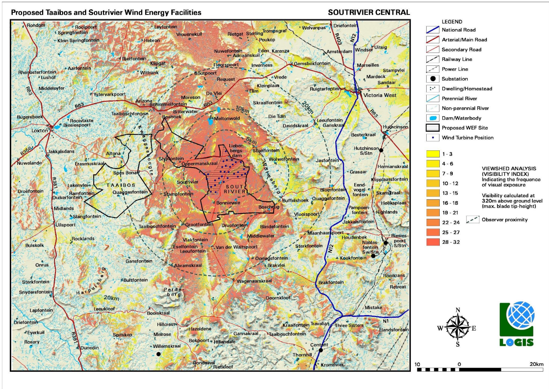
Map 4: Potential visual exposure (viewshed analysis) of the proposed Soutrivier Central WEF
