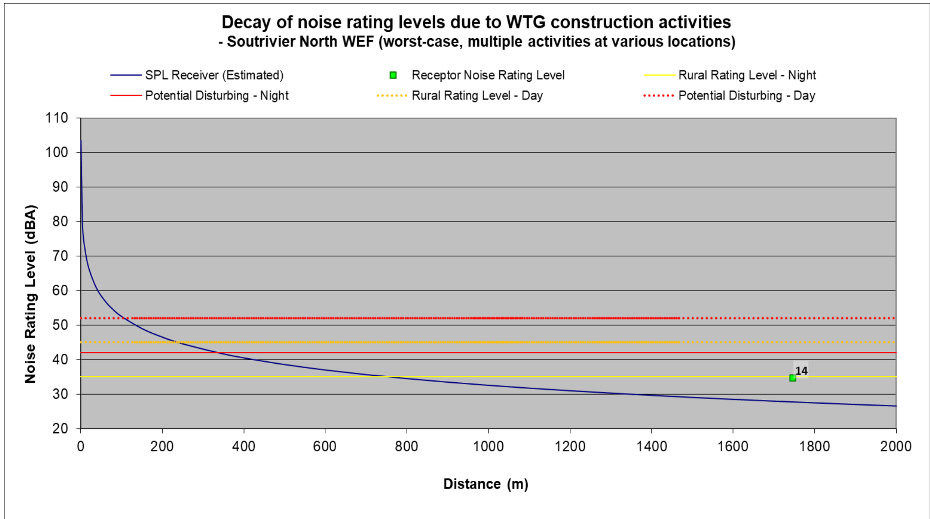
Figure 9-3: Projected conceptual construction noise levels – Soutrivier North WEF
