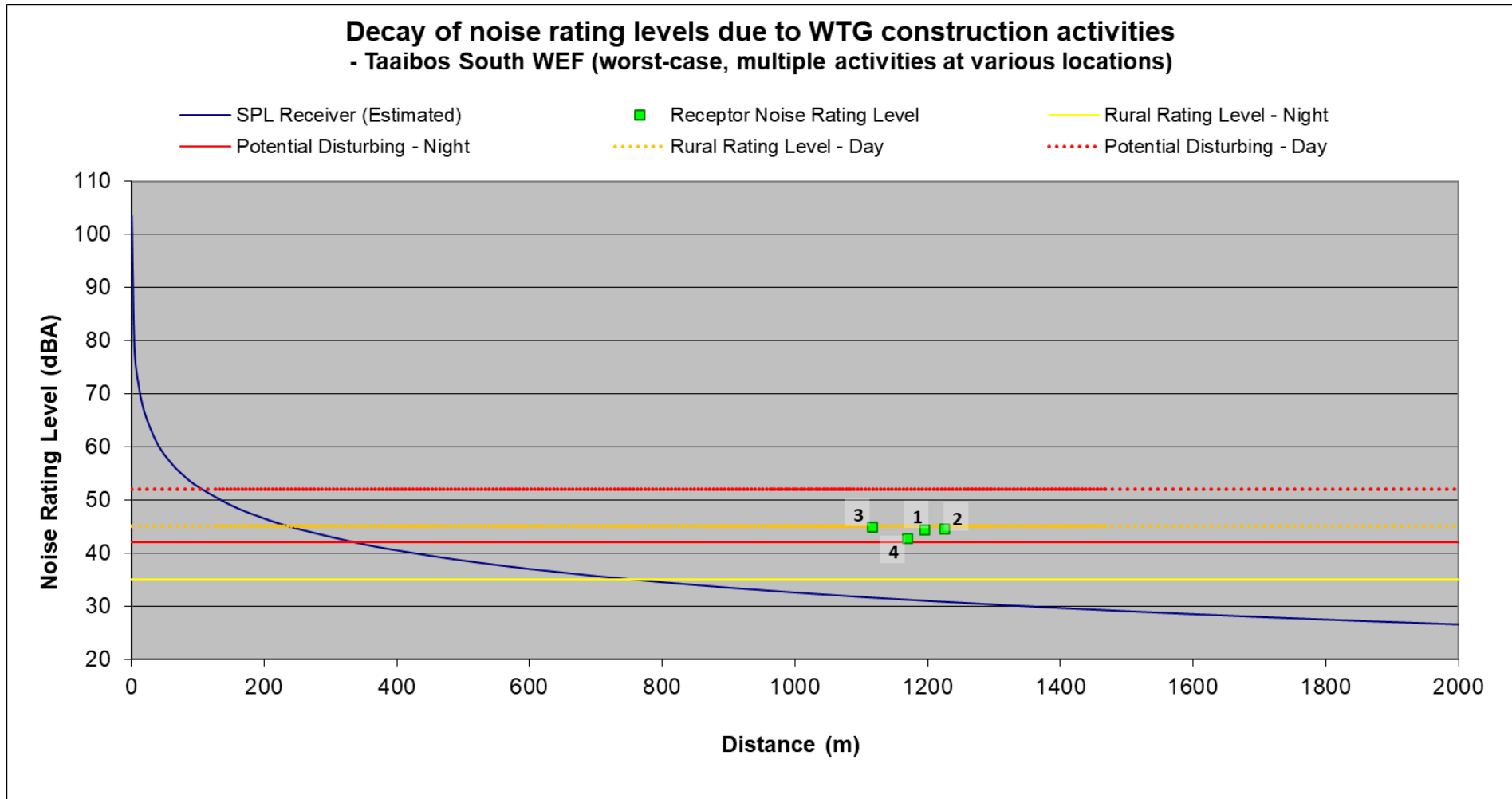
Figure 9-3: Projected conceptual construction noise levels – Taaibos South WEF
