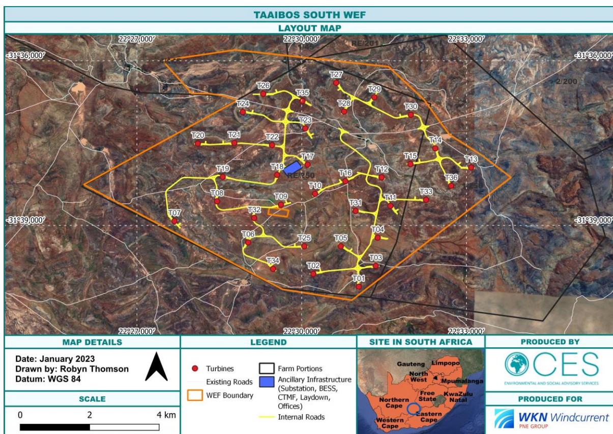
Figure 1: Layout Map of the Proposed Taaibos South WEF Development.
